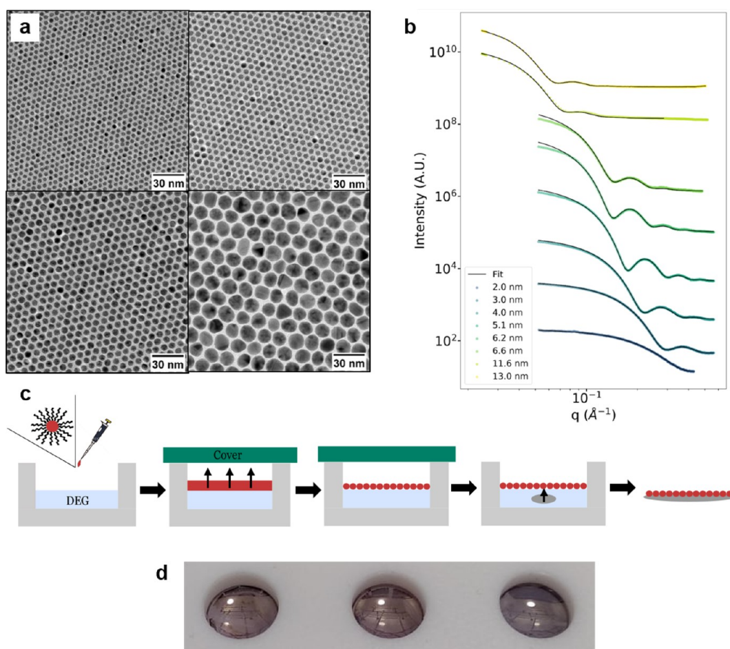
Figure 1. (a) TEM images of 4, 5, 6, and 14 nm Au NPs and (b) their SAXS diagrams fitted with a model of polydisperse spheres (solid black lines). (c) Schematic of the 2D self-assembly at the liquid/air interface of NPs into superlattices using a Teflon well. (d) NP thin films with mirror effect on DEG in the Teflon well after solvent evaporation.
