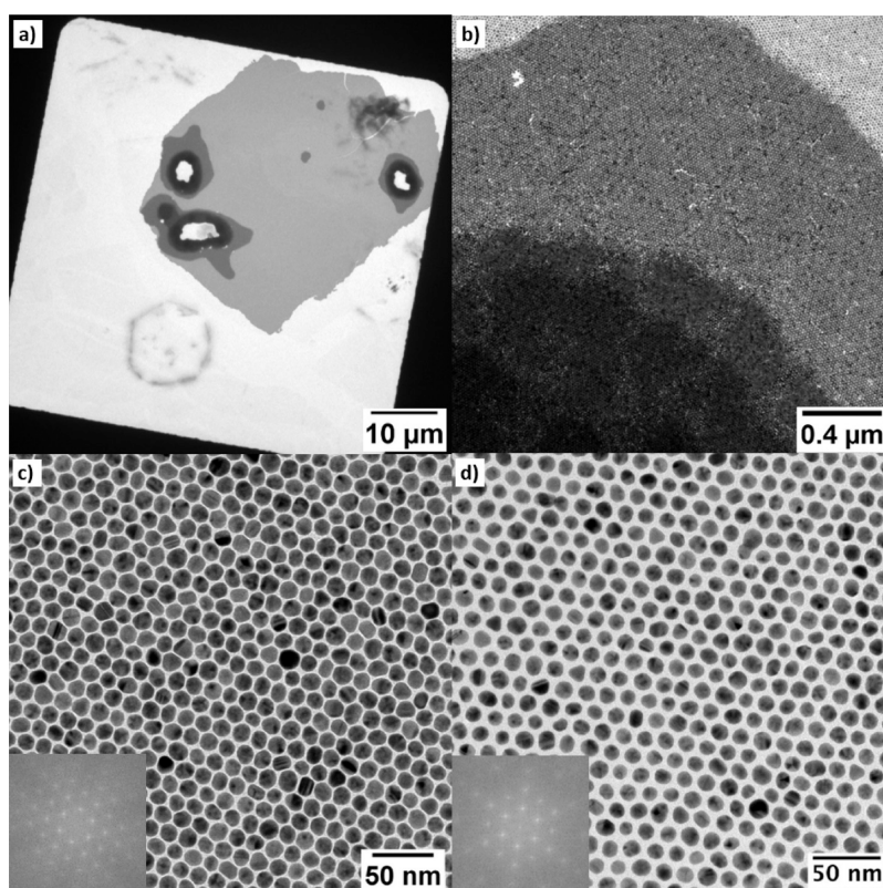
Figure 4. (a–c) TEM images of self-assembled 14 nm Au NPs. Low magnification of a film composed of a majority of monolayers (light area) and of bi- and multilayers (darkest areas) (a). Transition from a monolayer to multilayers (b). Hexagonal monolayers of 14 nm NPs coated with OLA (c) and 11.3 nm NPs coated with PSSH (d).
