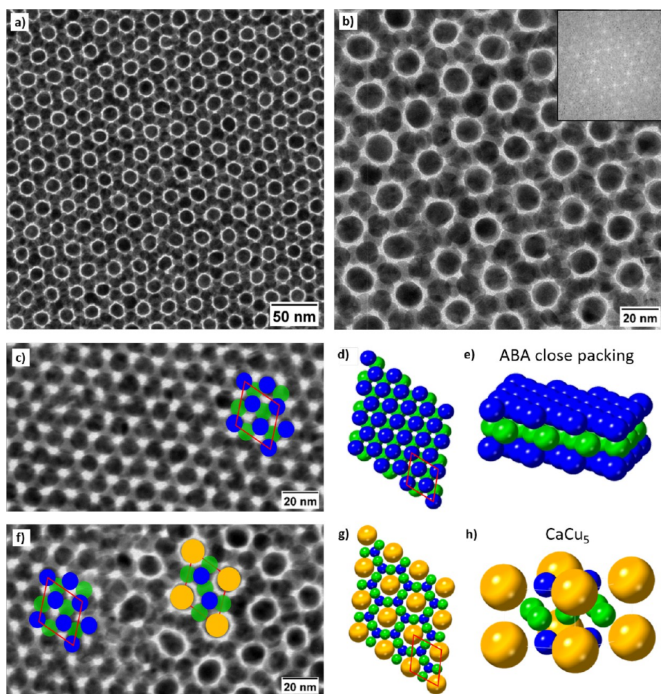
Figure 6. TEM images and models of self-assembled 11.3 nm Au NPs coated by PSSH. (a and b) Binary hexagonal \text{CaCu}_5 phase ( P6/mmm group); the inset shows the Fourier transformed image. (c) Three hexagonal layers of “small” NPs packed in an ABA sequence and (d) 2D and (e) 3D models. (f) TEM image showing the insertion of the “large” NPs into the ABA packing structure. (g) 2D and (h) 3D models of the binary \text{CaCu}_5 phase.
