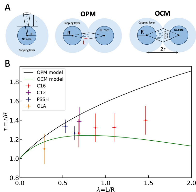
Figure 5. (A) Description of the OPM and the OCM models with the relevant notations. (B) Comparison of the OCM and OPM models relating the \tau and \lambda parameters with the experimental results for gold NP monolayers with different ligands: hexadecanethiol (C16), dodecanethiol (C12), thiolated polystyrene (PSSH), and oleylamine (OLA).
