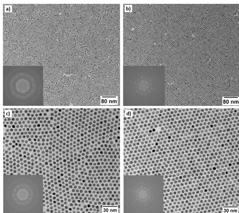
Figure 3. Effect of added thiol in solution for 6 nm nanoparticles: (a, c) short-range ordered films without thiols, (b, d) long-range ordered films with thiols.
