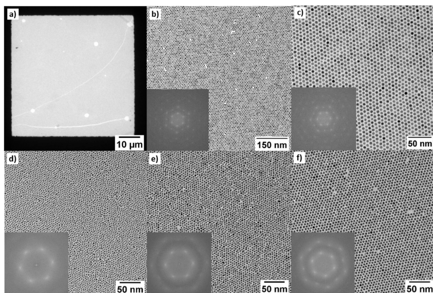
Figure 2. TEM images of self-assembled Au NPs of different sizes. (a) Low-resolution TEM image showing the homogeneity of the film composed of 6.4 nm Au NPs over very long distances (around 50 \mu\text{m} ). (b and c) Hexagonal lattice of 6.4 nm gold NPs. TEM images of self-assembled Au NPs of (d) 3 nm, (e) 4 nm, and (f) 5 nm.
