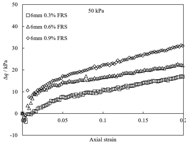
Figure 3. Variations of deviator stress increment of fibre reinforced soil with different fibre inclusion ratios at 50 kPa confining pressure.
