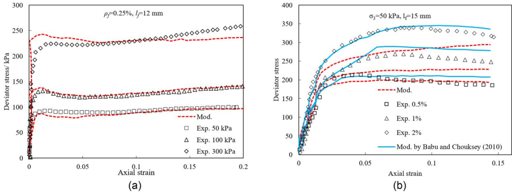
Figure 13. Predicted results via the proposed model and experimental results of stress-strain relationships in (a) Corriea et al. (2021) (b) Babu and Chouksey (2010).
