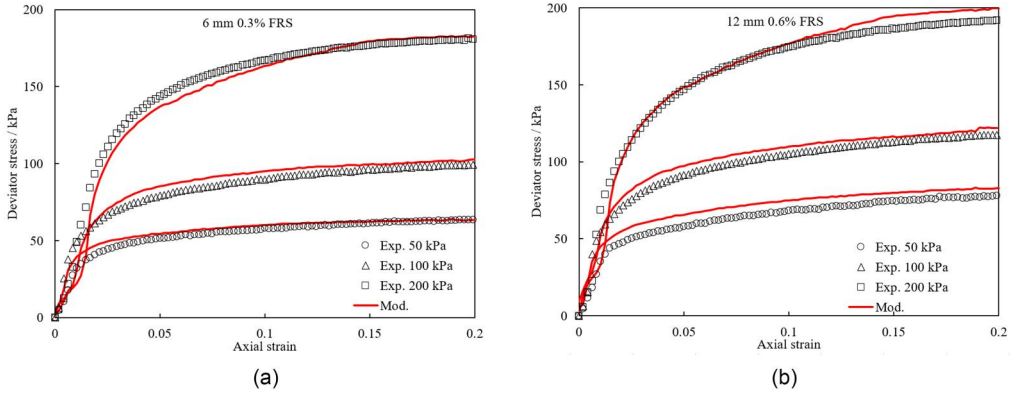
Figure 12. Predicted and experimental results of stress-strain relationships of fibre reinforced clay in this study with (a) l_f = 6 mm, \rho_f = 0.3\% (b) l_f = 12 mm, \rho_f = 0.6\% .
