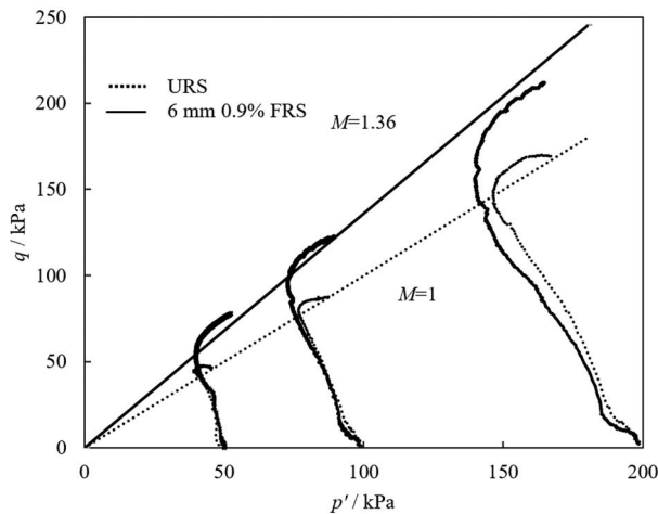
Figure 6. Stress paths in p' - q plane of unreinforced soil and selected fibre reinforced soil ( l_f = 6 \text{ mm} , \rho_f = 0.9\% ) at different confining pressures.
