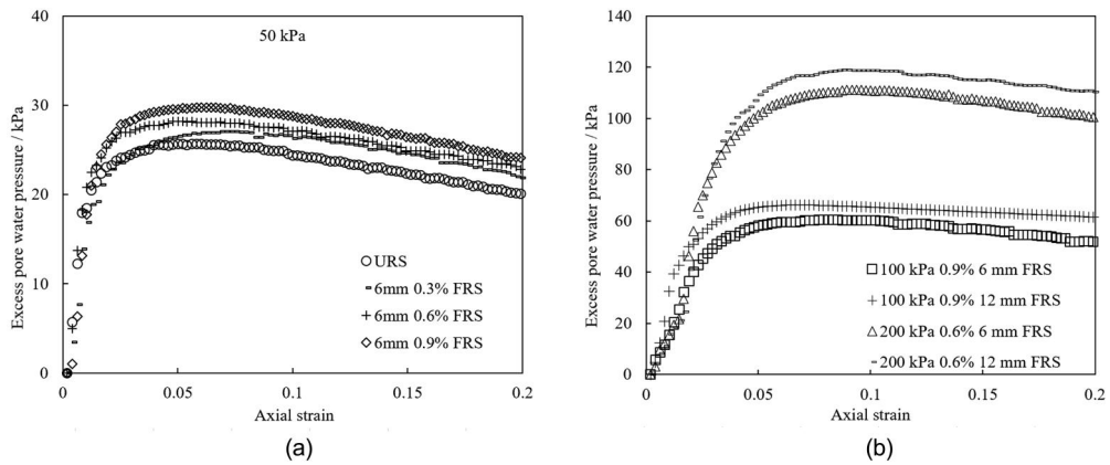
Figure 5. Pore water pressure-strain relationships of selected fibre reinforced specimens with different (a) fibre inclusion ratio (b) fibre inclusion ratio, fibre length and confining pressure.
