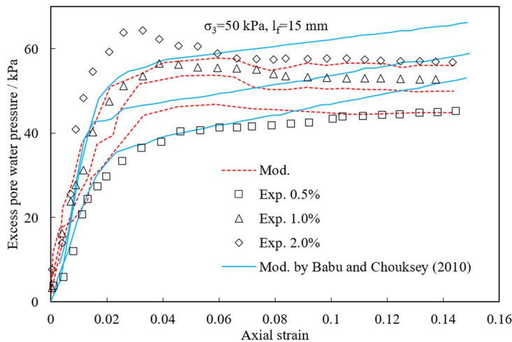
Figure 15. Predicted results via the proposed model and experimental results of excess pore water pressure-strain relationships in Correia et al. (2021).
