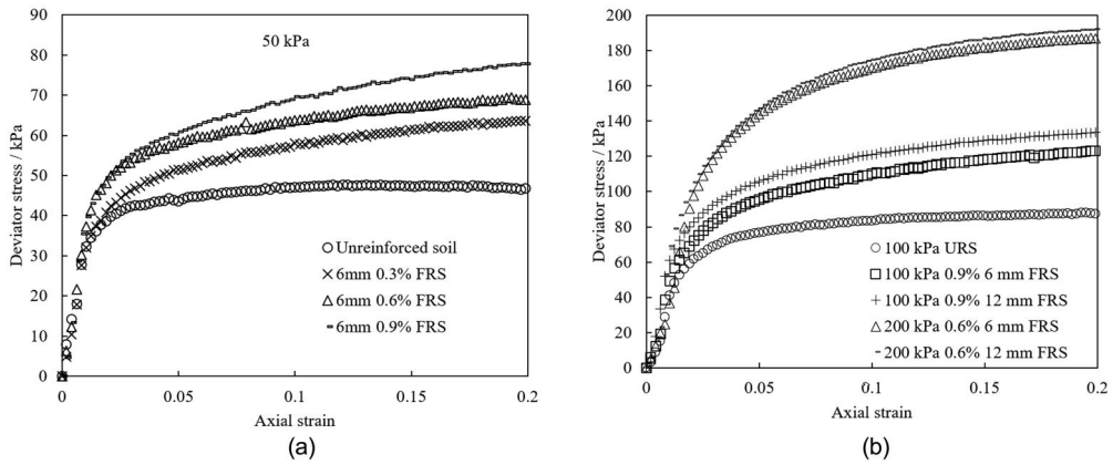
Figure 2. Deviator stress-strain relationships of selected fibre reinforced specimens with different (a) fibre inclusion ratios (b) fibre inclusion ratios, fibre lengths and confining pressures.
