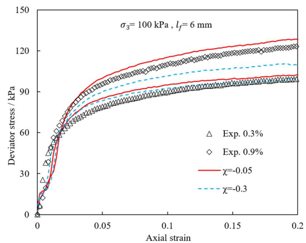
Figure 10. Influence of confining pressure parameter \gamma on the predicted results.
