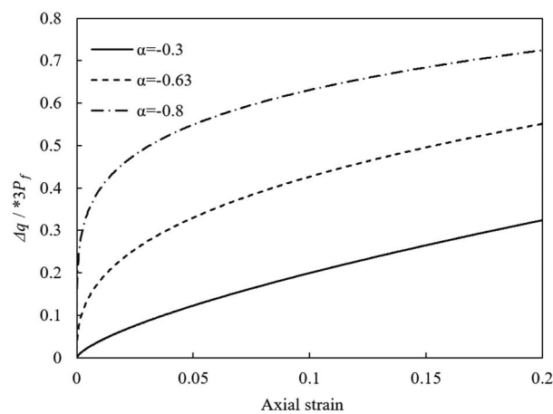
Figure 8. Variation of strength improvement trend with change of sliding parameter \alpha .
