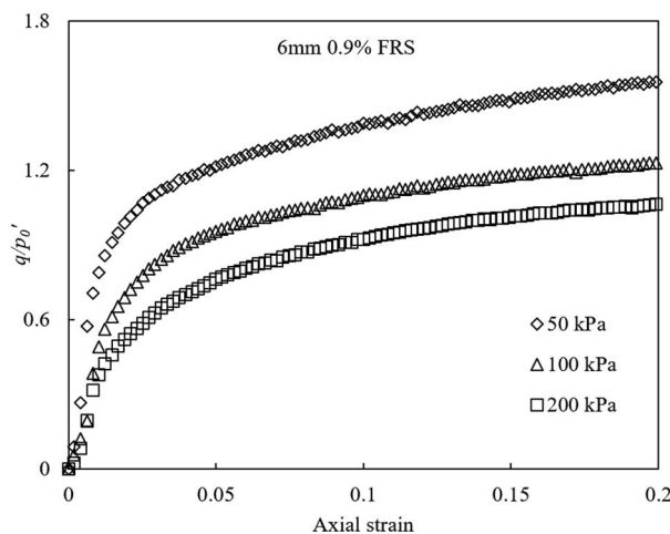
Figure 4. Normalised stress-strain curves of selected reinforced samples ( l_f = 6 mm, \rho_f = 0.9\% ).
