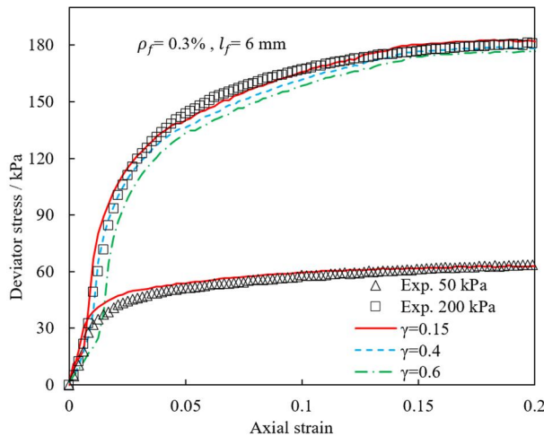
Figure 11. Influence of fibre inclusion ratio parameter \chi on the predicted results.
