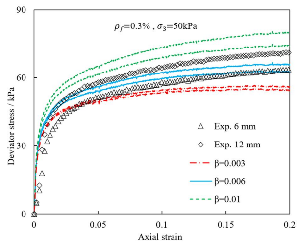
Figure 9. Influence of fibre length parameter \beta on the predicted results.
