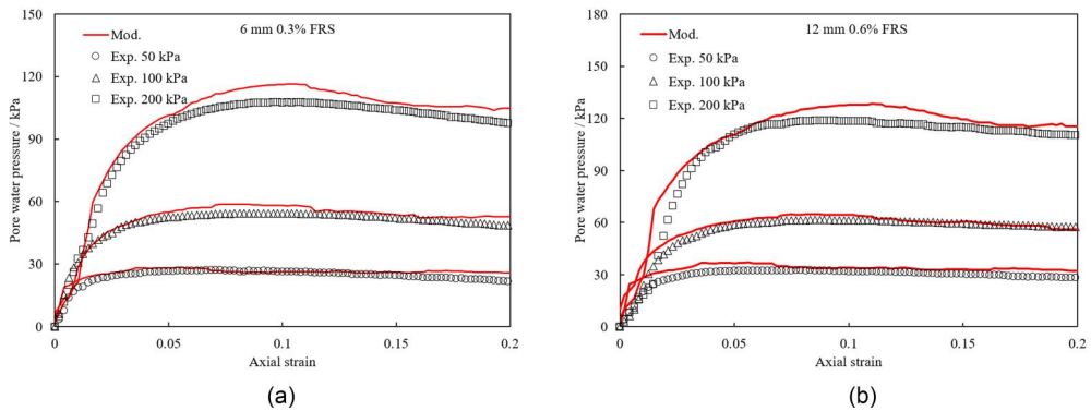
Figure 14. Predicted and experimental results of excess pore water pressure-strain relationship of fibre reinforced clay in this study with (a) l_f = 6 mm, \rho_f = 0.3\% (b) l_f = 12 mm, \rho_f = 0.6\% .
